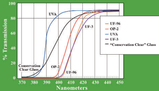
Comparison of UV Filtering Materials 0.250 inches thick
